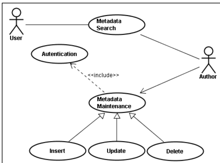
Figure 1 – DIS use-cases
